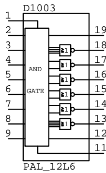
PAL_12L6 D????
