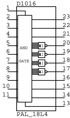
PAL_18L4 D?????
