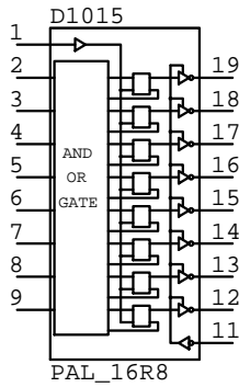
PAL_16R8 D?????
