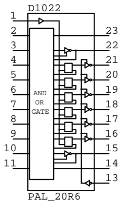
PAL_20R6 D?????
