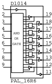
PAL_16R6 D?????
