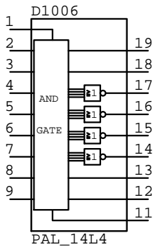
PAL_14L4 D????
