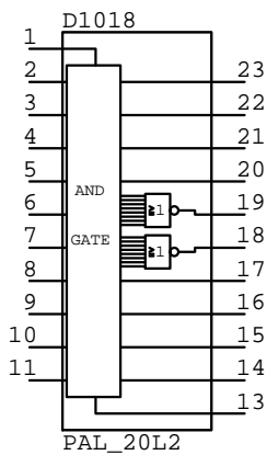
PAL_20L2 D?????
