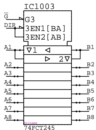
74FCT245 IC????
