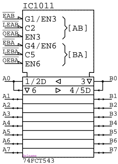
74FCT543
