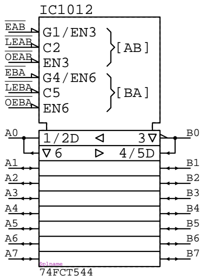
74FCT544
