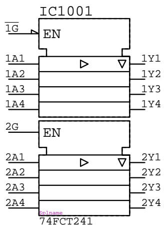
74FCT241 IC????
