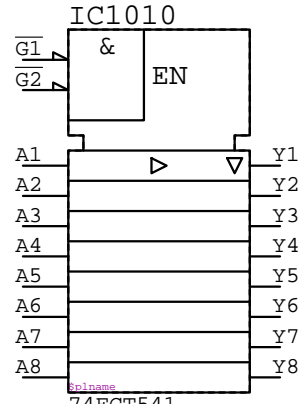
74FCT541 IC????
