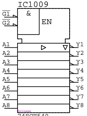
74FCT540 IC????
