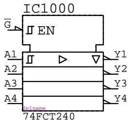
74FCT240 IC????
