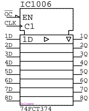
74FCT374 IC????
