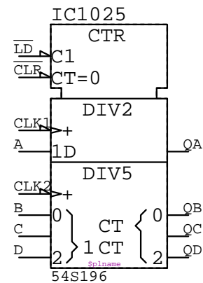
54S196 IC????
