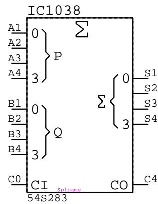
54S283 IC????
