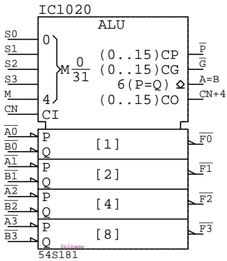
54S181 IC????
