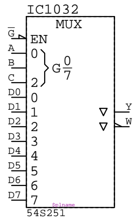
54S251 IC????
