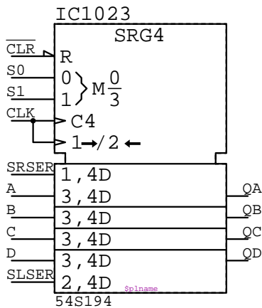
54S194 IC????
