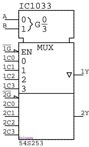
54S253 IC????
