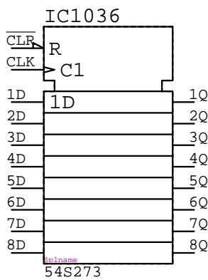
54S273 IC????
