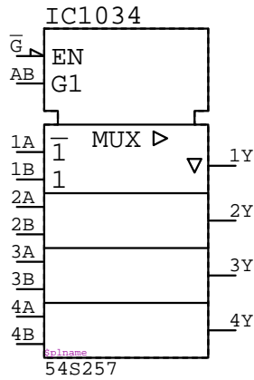
54S257 IC????
