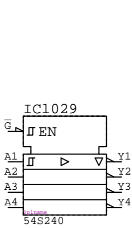
54S240 IC????
