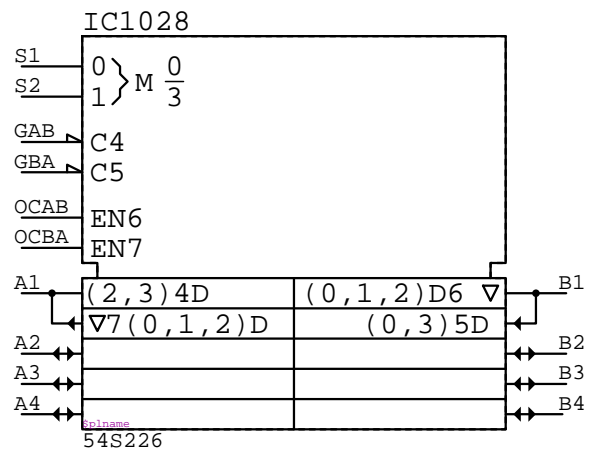
54S226 IC????
