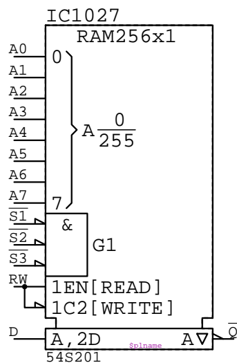
54S201 IC????
