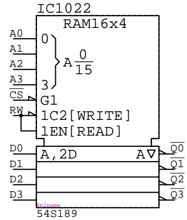
54S189 IC????
