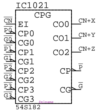
54S182 IC????
