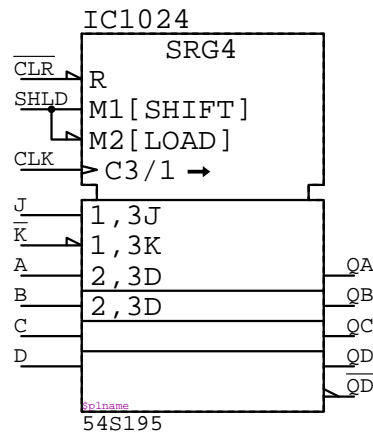
54S195 IC????
