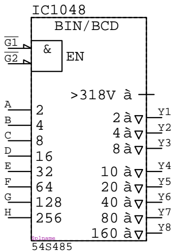
54S485 IC????
