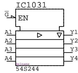
54S244 IC????
