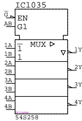
54S258 IC????
