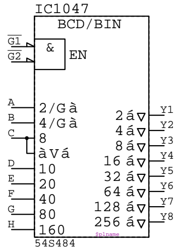
54S484 IC????
