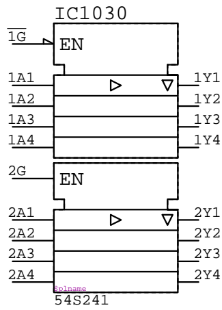
54S241 IC????
