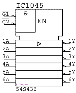
54S436 IC????
