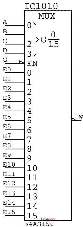
54AS150 IC????
