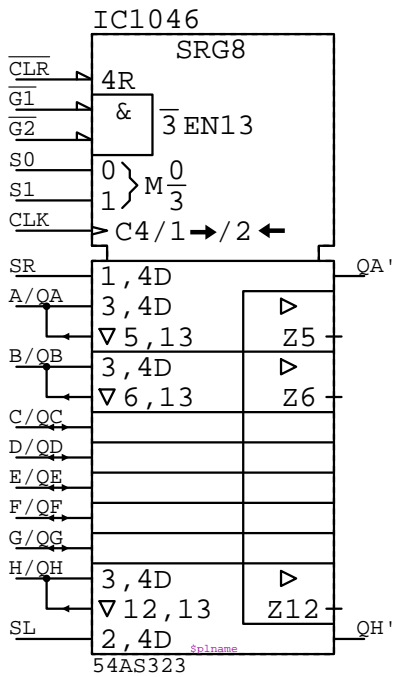
54AS323 IC?????
