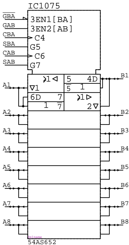
54AS652 IC?????
