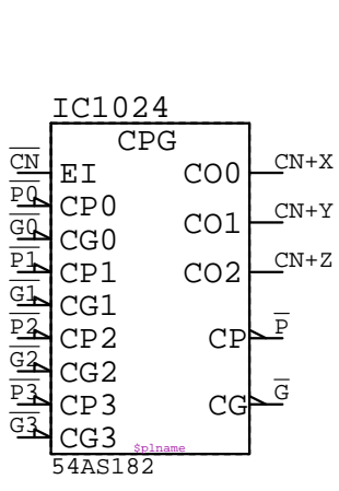
54AS182 IC????
