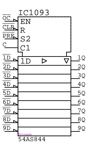
54AS844 IC????
