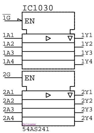
54AS241 IC????
