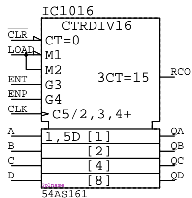
54AS161 IC????
