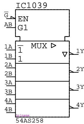
54AS258 IC????
