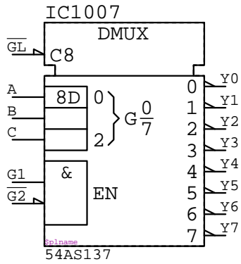
54AS137 IC????
