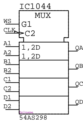
54AS298 IC?????
