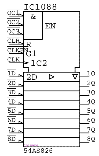
54AS826 IC????
