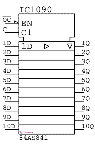
54AS841 IC????
