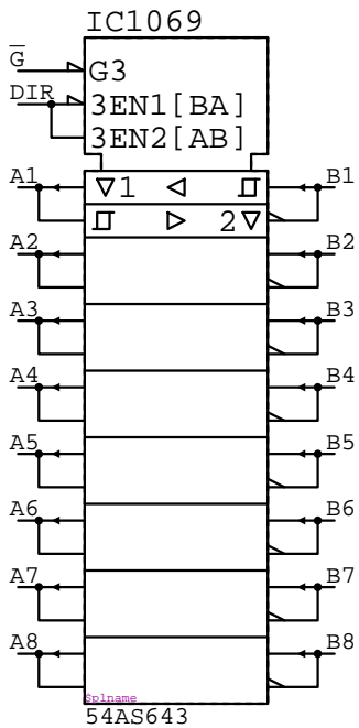
54AS643 IC?????
