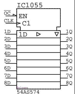
54AS574 IC?????
