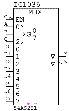
54AS251 IC????
