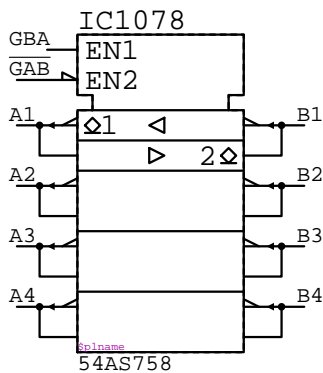
54AS758 IC?????
