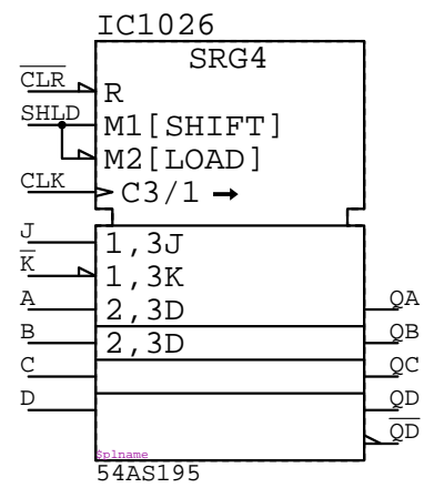
54AS195 IC????
