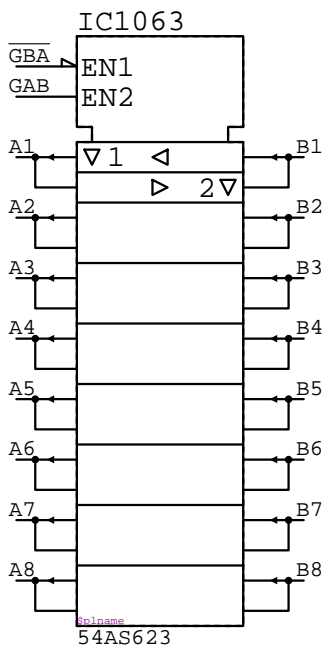
54AS623 IC????
