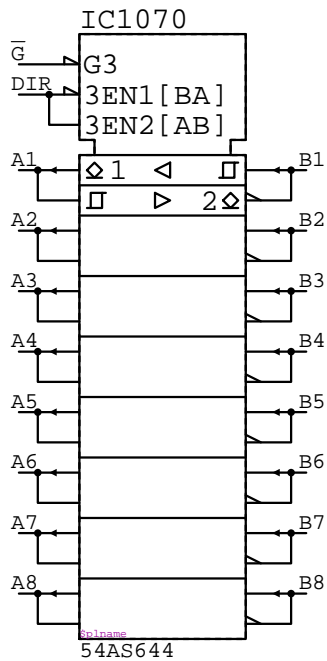
54AS644 IC?????
