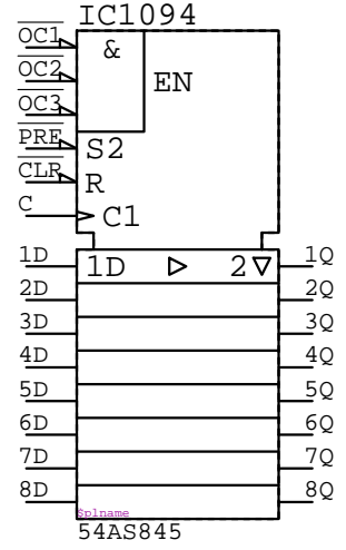
54AS845 IC????
