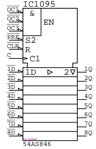
54AS846 IC????
