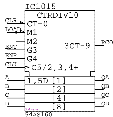
54AS160 IC????
