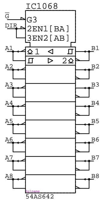
54AS642 IC????
